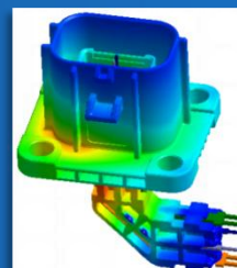
Mold Flow
