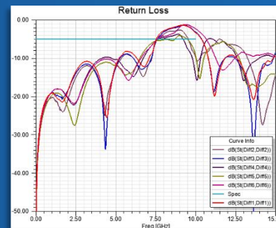
signal integrity
