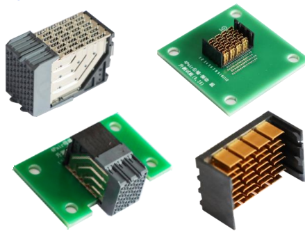
high speed backplane conn
